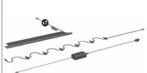
2', 3' or 4' Universal Downlight Kit – 7 pack Each kit includes 7 lights, power supply and power cord
